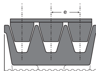
皮帶與滑輪 Belt & Pulley
